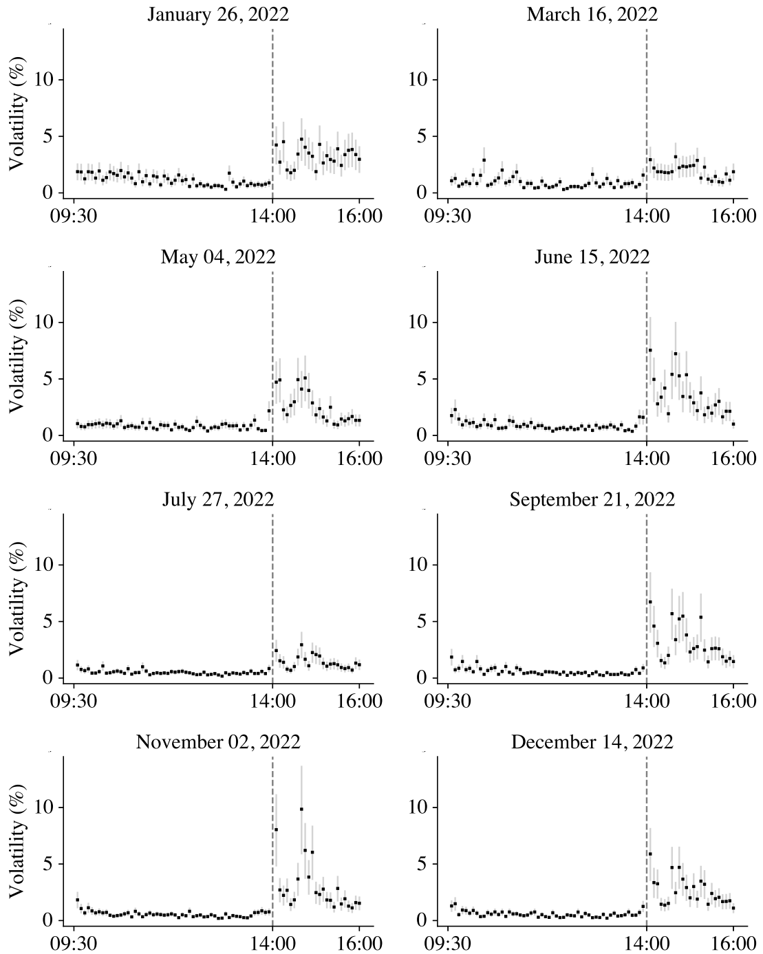
Fig. 4. Spot volatility estimates for the VOO ETF on FOMC announcement days. The figure plots the \hat{\sigma}_{\text{Stein}} spot volatility estimates based on 5-min VOO ETF candlesticks, expressed in daily percentage units. Pointwise confidence intervals at the 90% level is calculated as detailed in footnote 11. The vertical lines included in each of the panels indicate the official 14:00 FOMC announcement times.
